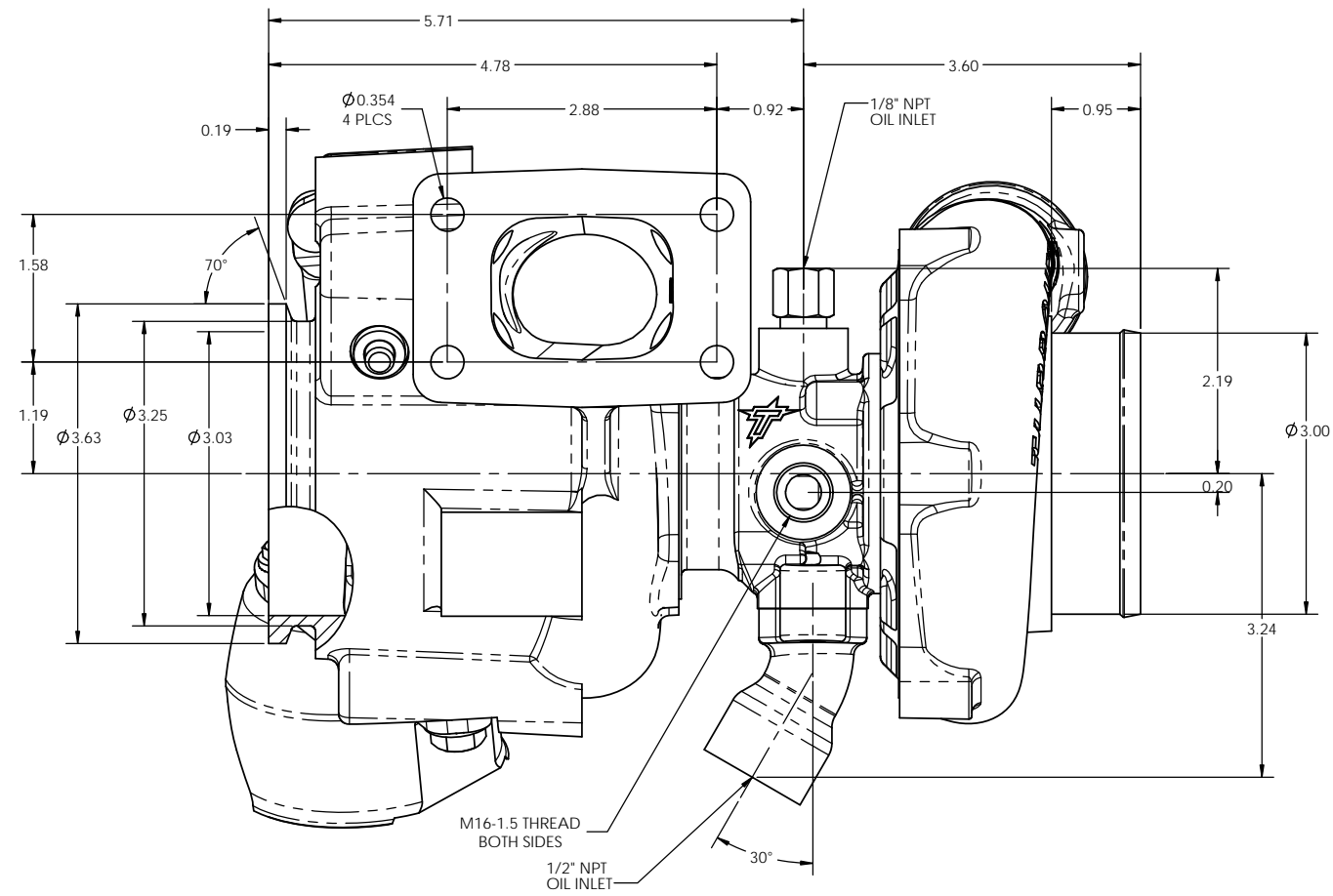
TURBOCHARGER, TNX-20/44 P/N 11814 WITH TURBINE HSG TNX-20 0.65 P/N 11796-1
