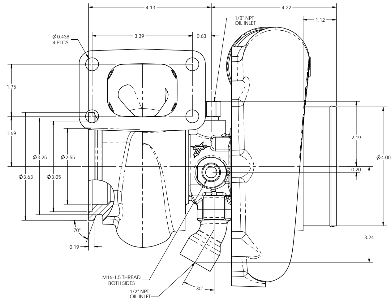
TURBOCHARGER, TNX-45/69 P/N 11901
