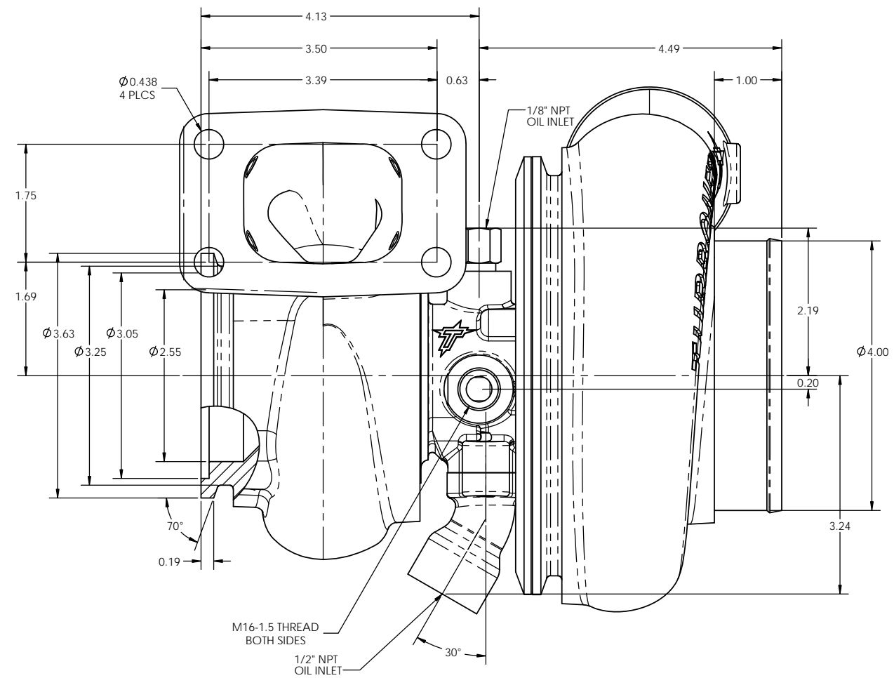
TURBOCHARGER, TNX-40/64 P/N 11900
