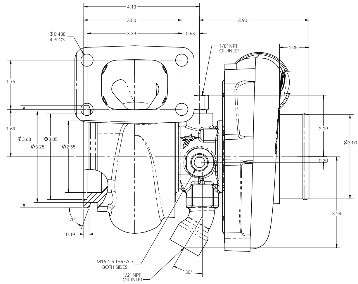
TURBOCHARGER, TNX-30/56 P/N 11899
