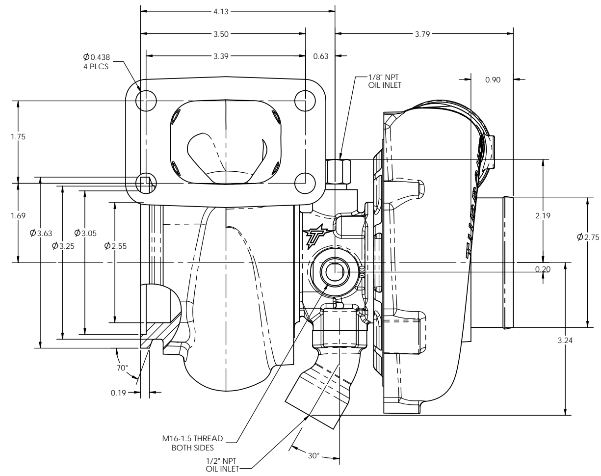
TURBOCHARGER, TNX-30/52 P/N 11898
