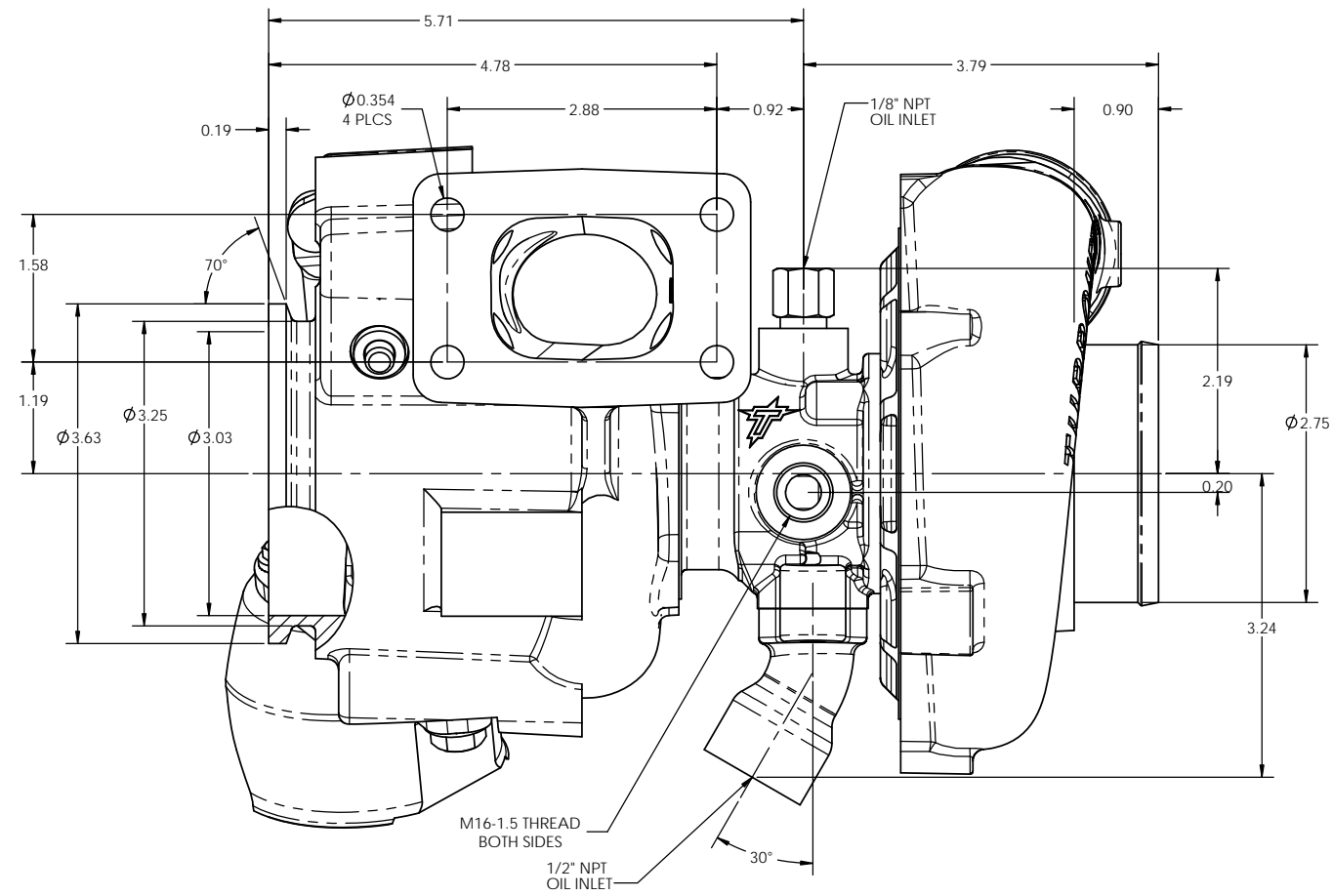
TURBOCHARGER, TNX-20/52 P/N 11815 WITH TURBINE HSG TNX-20 0.65 P/N 11796-1
