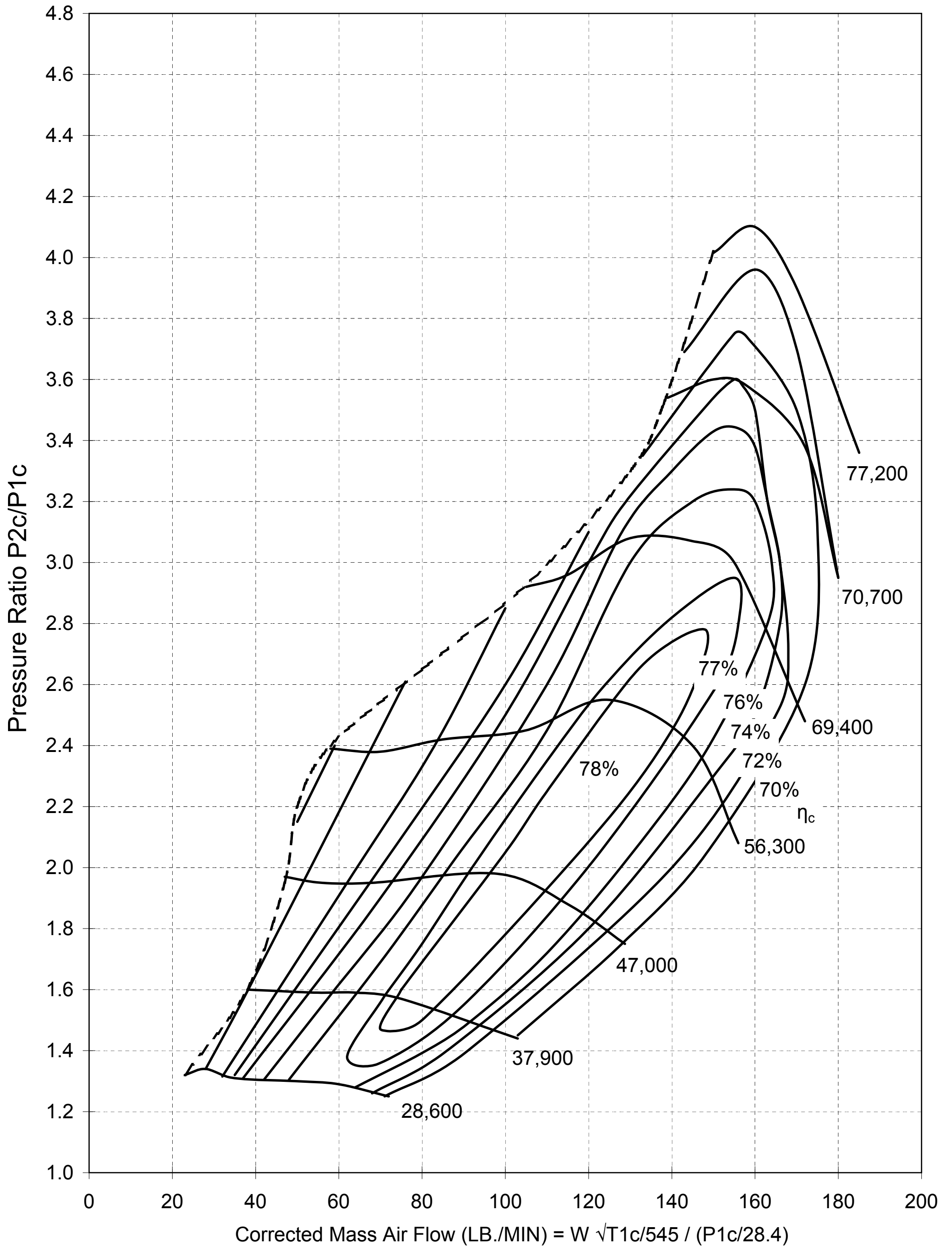
Turbonetics T-106
